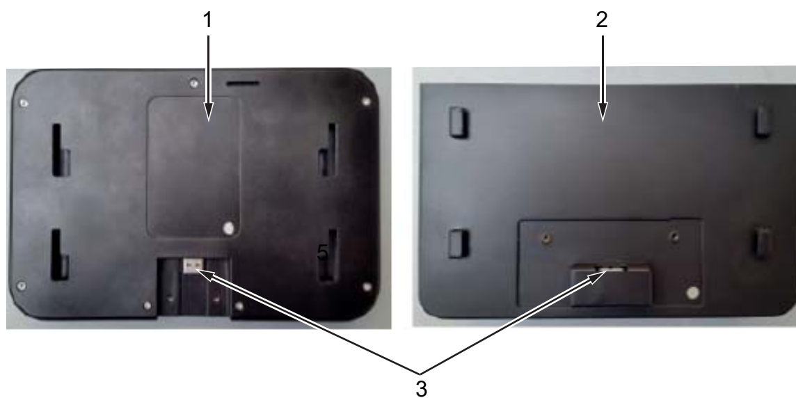
Figure 3-3: Display and Power Supply Unit
