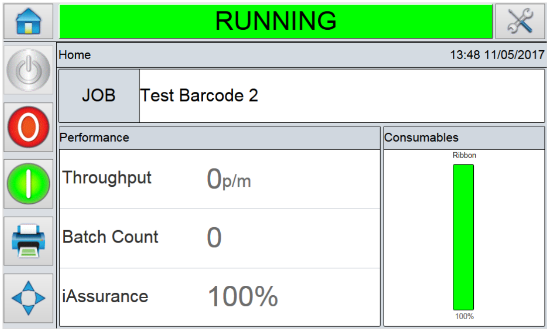
Figure 4-5: CLARiTY Home Screen in the Running State
