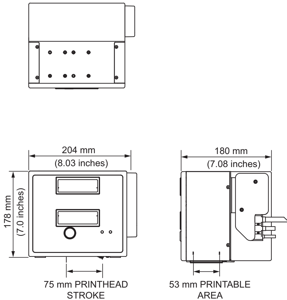
Figure A-2: Videojet DataFlex 6330 53mm LH Printer Dimensions
