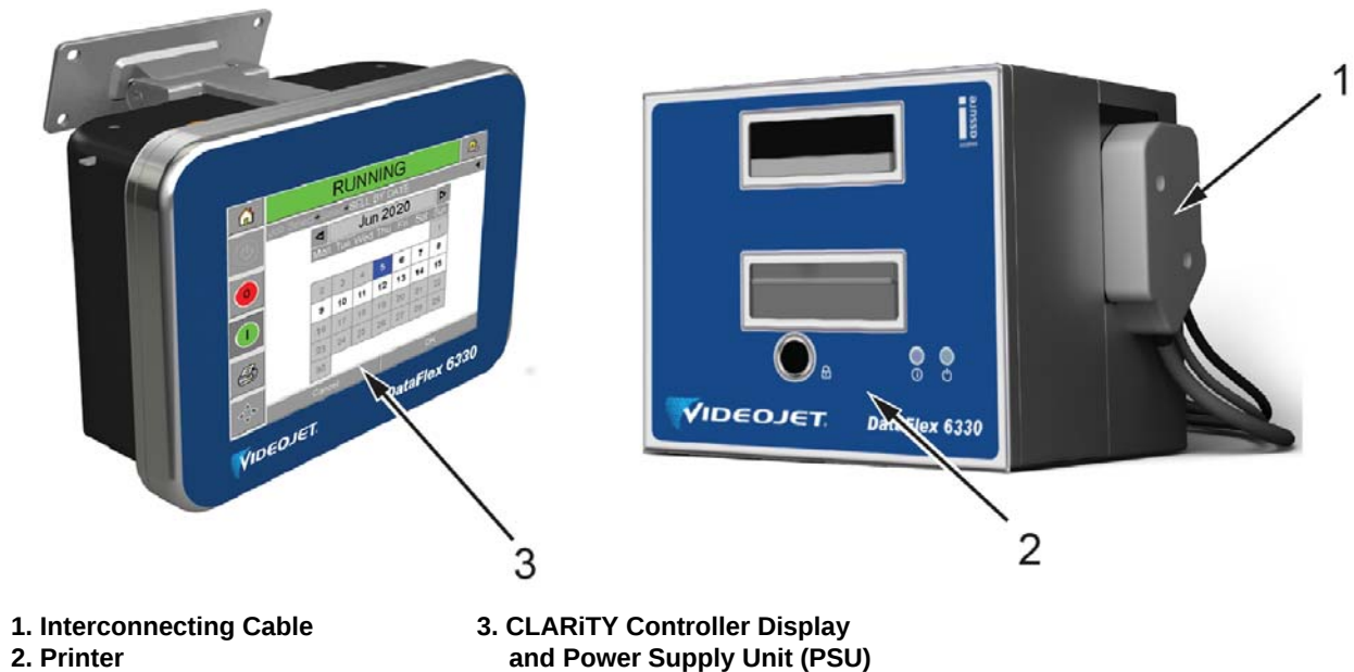
Figure 1-1: Videojet DataFlex 6330 Printer and CLARiTY Controller Display
